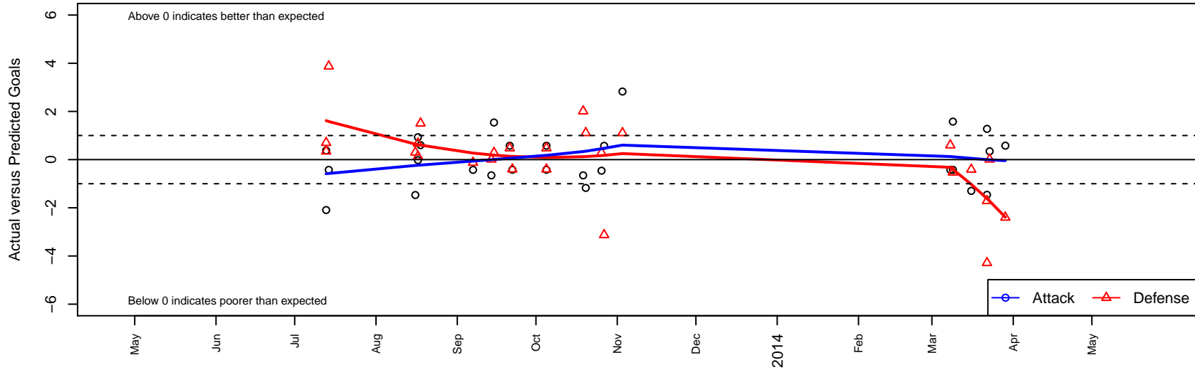
ASE Emerald Synergy G99 Dots are actual minus expected GF (blue circles) and GA (red triangles). Blue line is smoothed change in attack strength. Red is smoothed change in defense strength.
